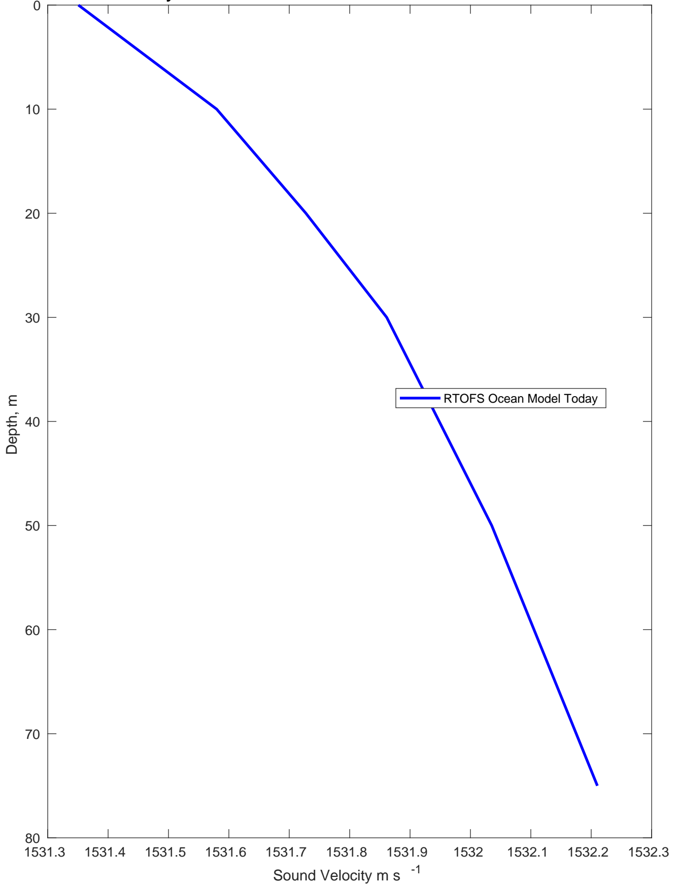
Sound Velocity Profile for Flower Gardens NMS on 08-Dec-2020 00:00:00
